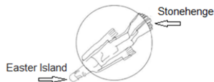
Figure1 – Earth model, Source: https://xxxxx.org
